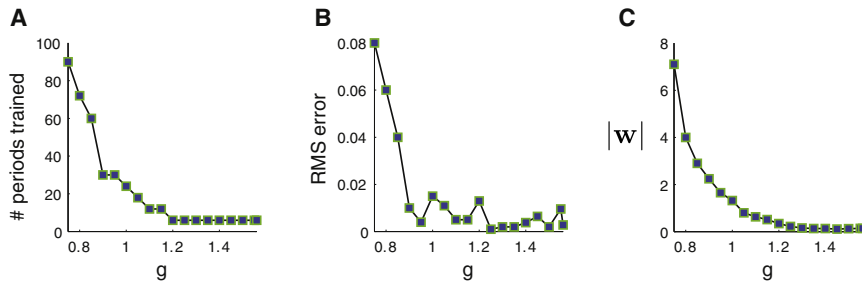
Figure 5. Chaos Improves Training Performance
